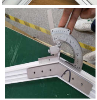
Cut 144.32°
