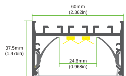
Aluminum diffuser
