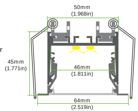
Aluminum diffuser
