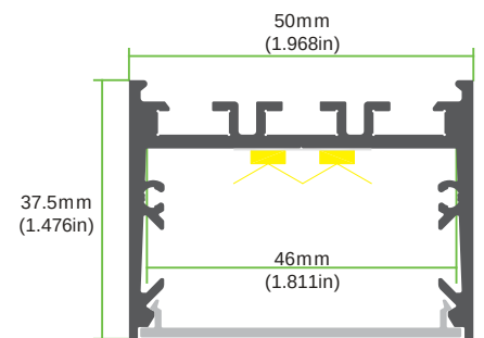
Aluminum diffuser
